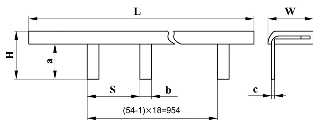
C45-1P-63-PIN
